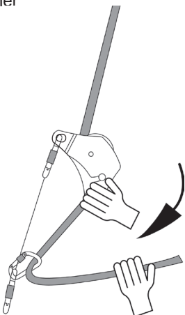
Tail rope through a carabiner
