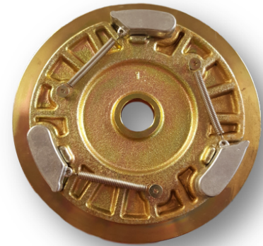
Triple pawl brake system
