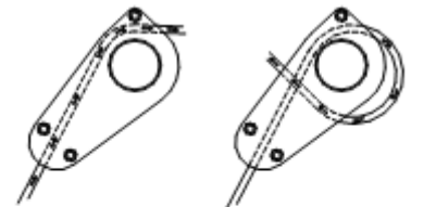
Rope round turn on the load positioner
