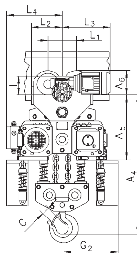
Model CPE/CPEF with integrated electric trolley, 10000 kg
