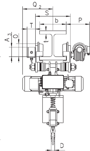
Model CPE/CPEF with integrated electric trolley, 10000 kg
