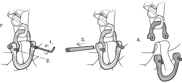
Gated ventral attachment point / Point d'attache ventral ouvrable
